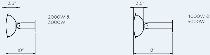
2000W SERIES
