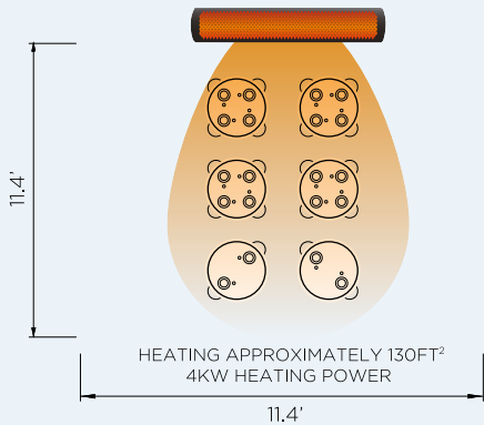
4000W SERIES
