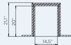
2000W & 4000W
